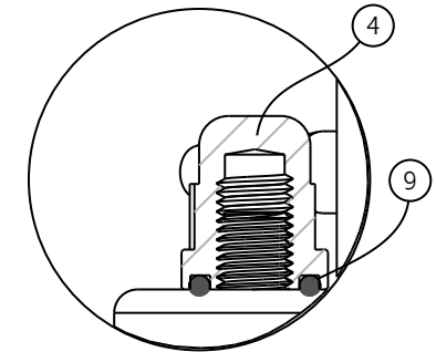
DETAIL A SECTION D-D
